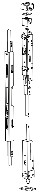
60 SERIES (Narrow Stile) Top and Bottom Rod 61 SERIES (Narrow Stile) Top Rod Only for Aluminum Doors
