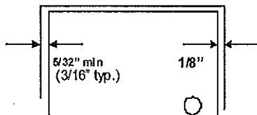
SINGLE DOOR
